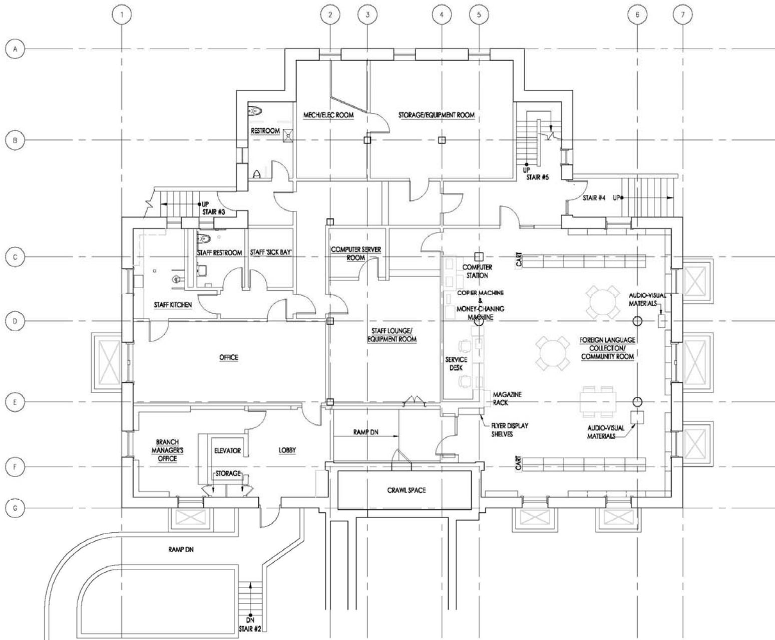
Existing Lower Level Floor Plan
