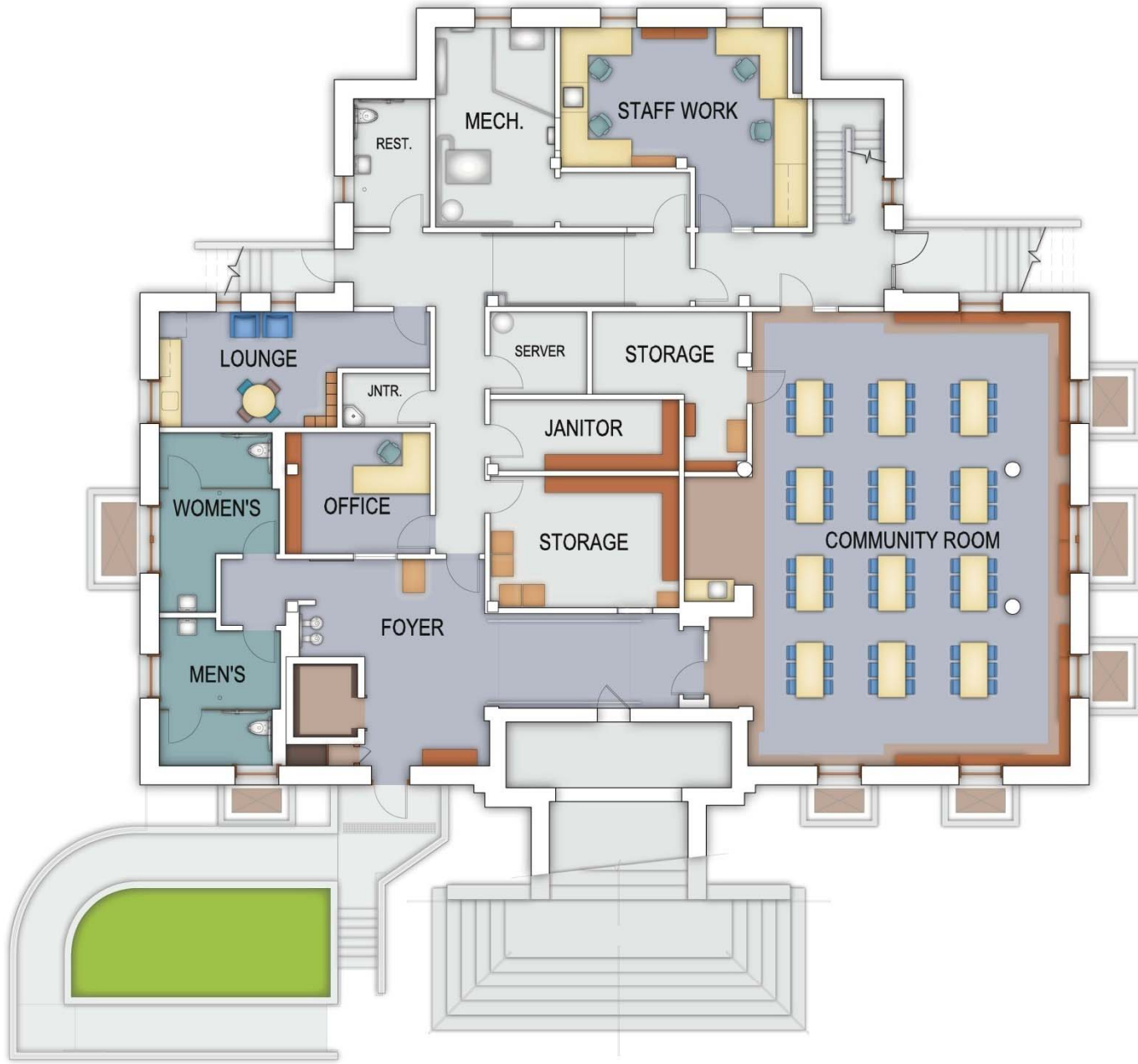
Proposed Lower Level Floor Plan
