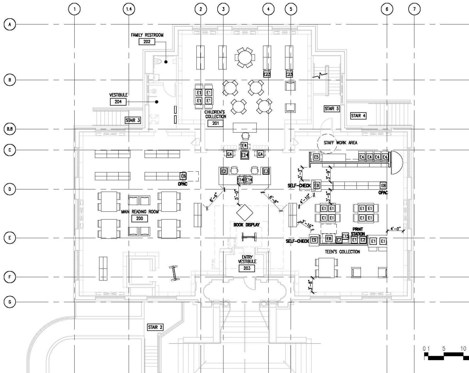
Proposed Upper Level Floor Plan
